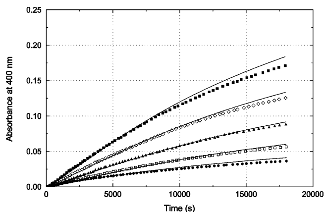
Figure 7. Chloride dependence of the measured (symbols) and calculated (solid lines) absorbances at pH = 5.35, [ClO_2^-]_0 = 5.0 mM, [S_4O_6^{2-}]_0 = 0.3 mM. [Cl^-]_0 (mM) = 0.0 (●), 1.0 (◻), 3.0 (▲), 6.0 (◇), and 10.0 (■).
