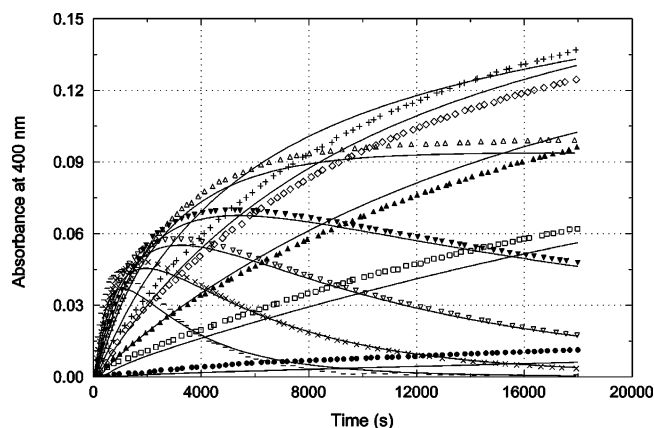
Figure 6. Measured (symbols) and calculated (solid lines) absorbances at pH = 5.07 and [ClO_2^-]_0 = 5.0 mM in the absence of chloride ion. [S_4O_6^{2-}]_0 (mM) = 0.1 (●), 0.14 (◻), 0.2 (▲), 0.3 (◇), 0.5 (+), 0.9 (△), 1.4 (▼), 2.0 (▽), 3.0 (×), and 5.0 (–).
