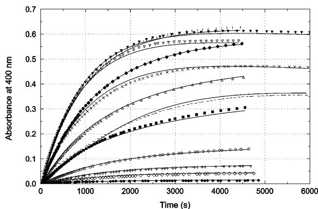
Figure 5. Measured (symbols) and calculated (solid lines) absorbances at pH = 4.65 and [S_4O_6^{2-}]_0 = 0.5 mM in the absence of chloride ion. [ClO_2^-]_0 (mM) = 0.5 (●), 1.4 (◇), 2.0 (+), 3.0 (○), 5.0 (■), 7.0 (△), 10.0 (◆), 14.0 (◻), 17.0 (▼), 20.0 (▽), 25.0 (×), and 30.0 (–).
